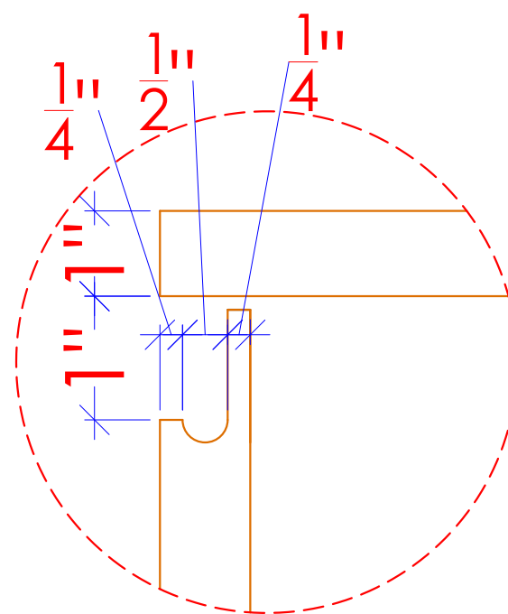
Detail A
