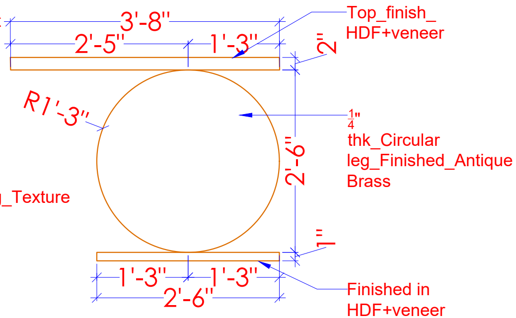
CONSOLE ELEVATION
