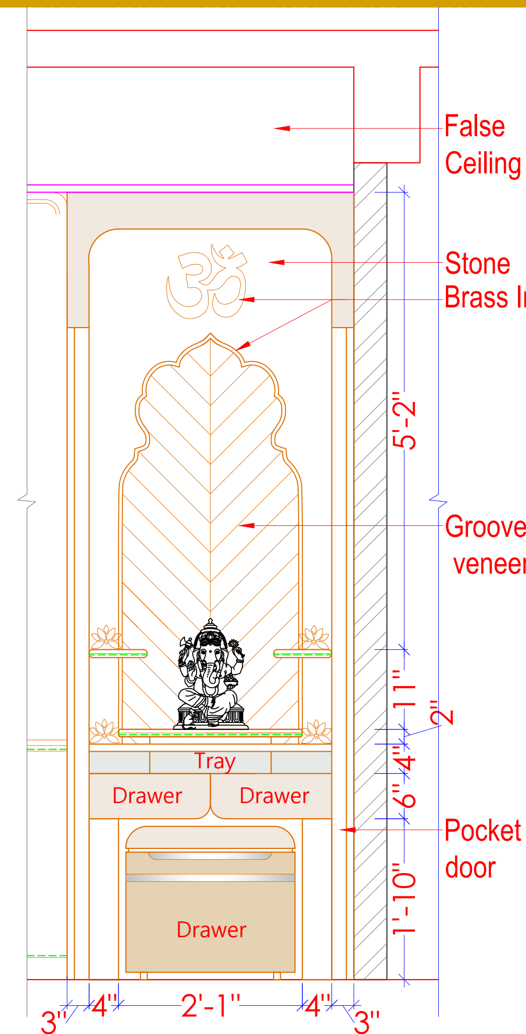
INTERNAL ELEVATION
