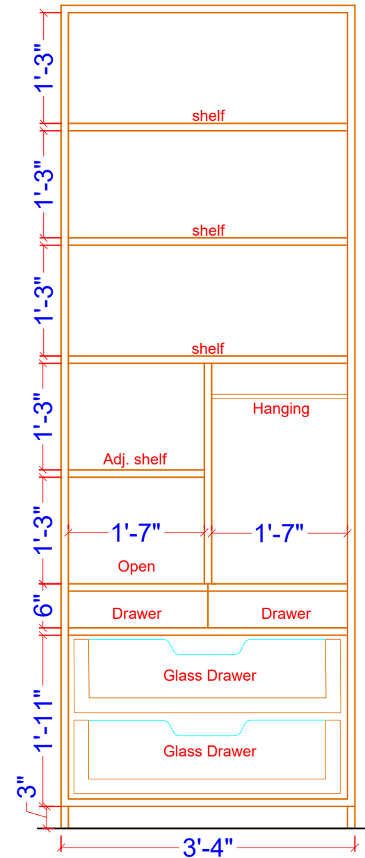
HIS WARDROBE INTERNAL DETAIL
