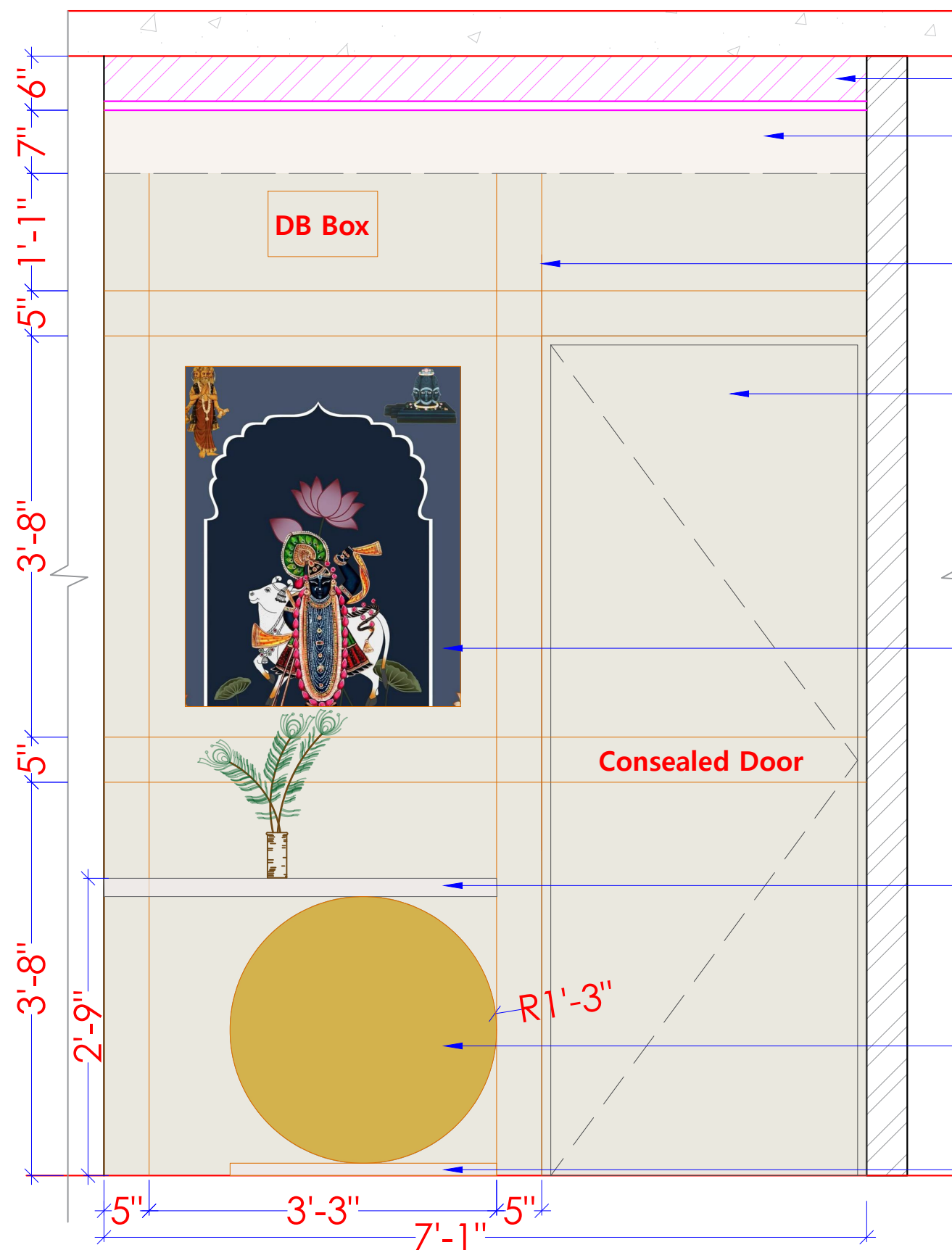
ELEVATION - AA'
