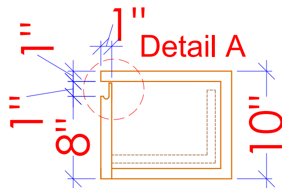
TV UNIT PLAN
