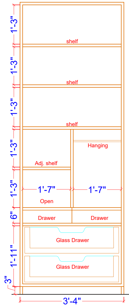
HER WARDROBE INTERNAL DETAIL
