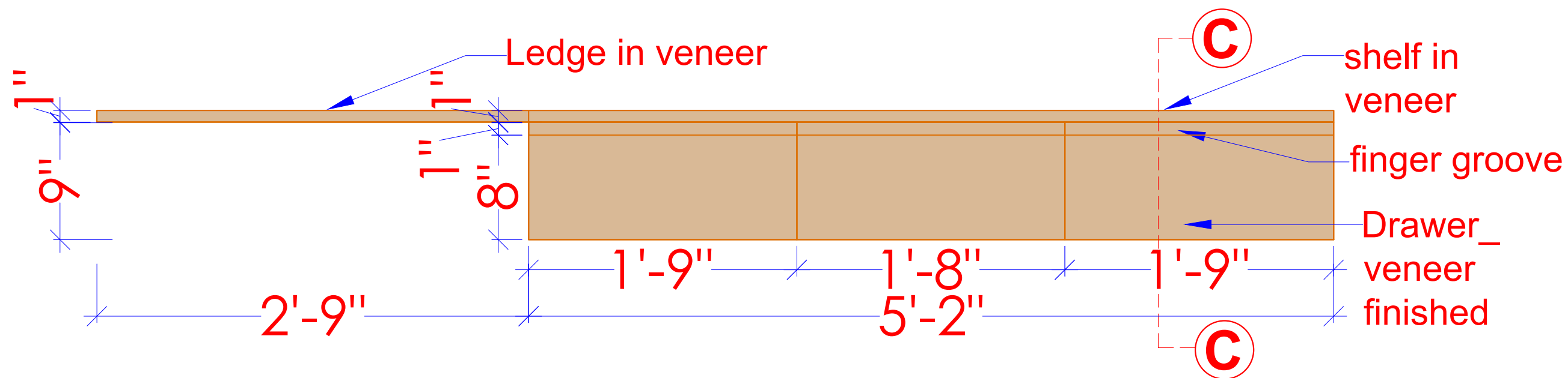
TV UNIT ELEVATION
