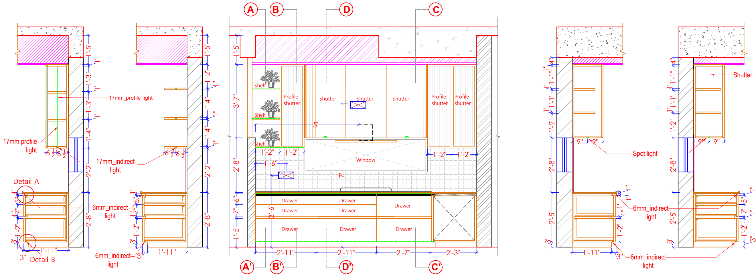
SECTION BB'
