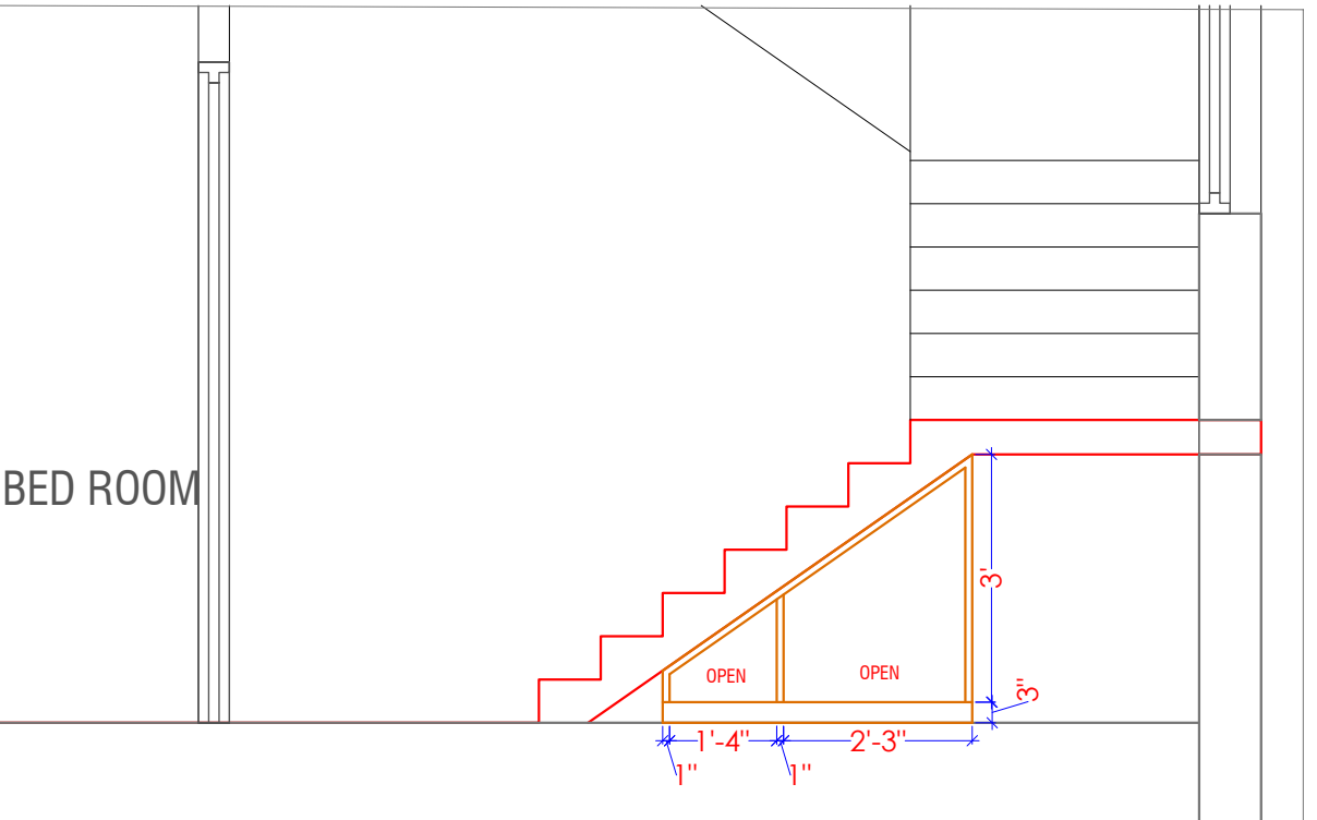
ELEVATION C
